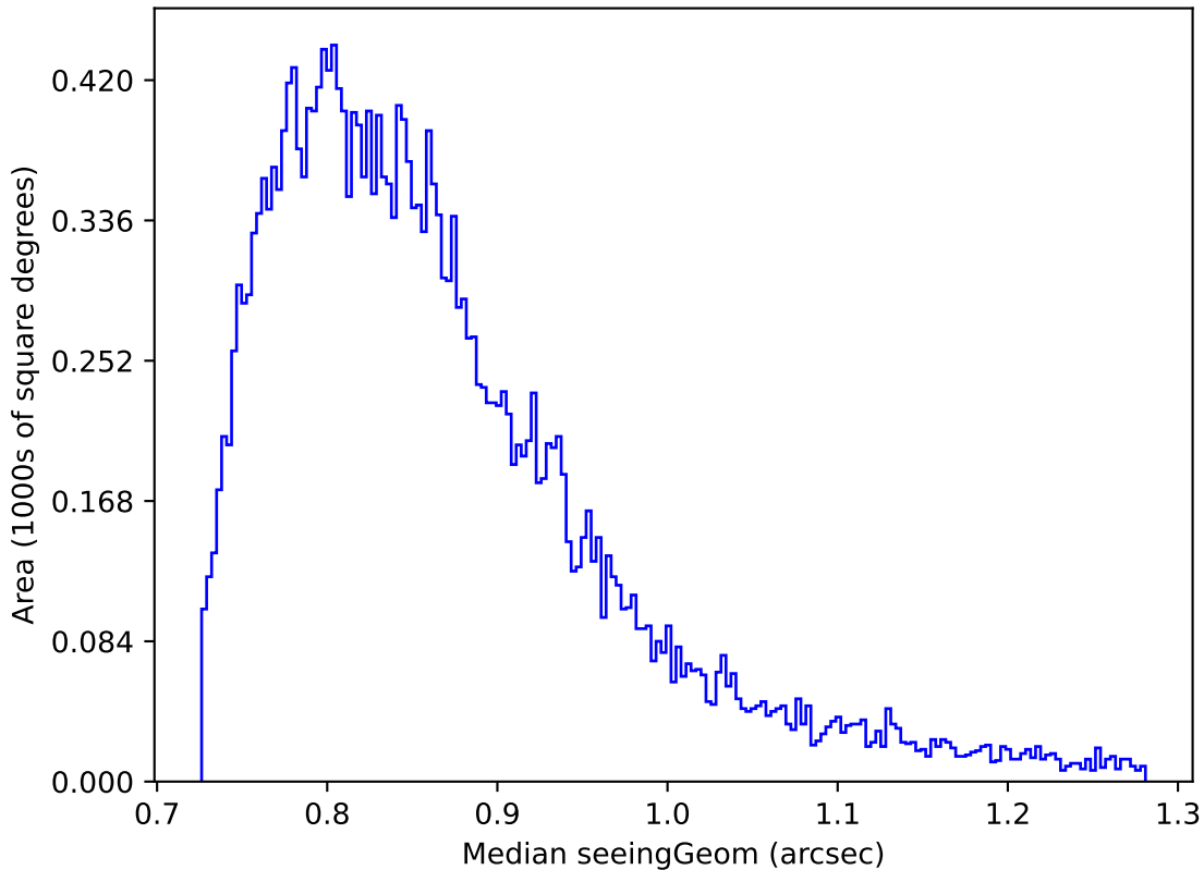
early_u_fpextra2.0_v3.4_10yrs Yr 1 all bands: Median seeingGeom
