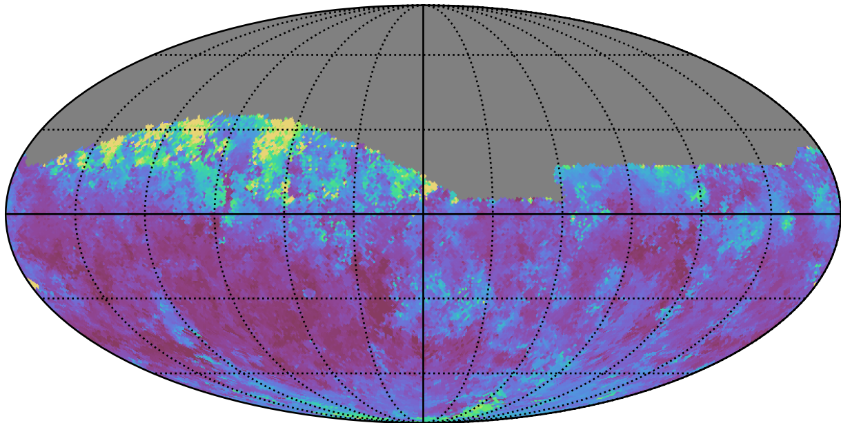
early_u_fpextra2.0_v3.4_10yrs Yr 1 z band: Median seeingEff
