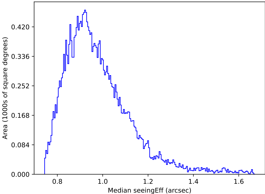
early_u_fpextra2.0_v3.4_10yrs Yr 1 z band: Median seeingEff
