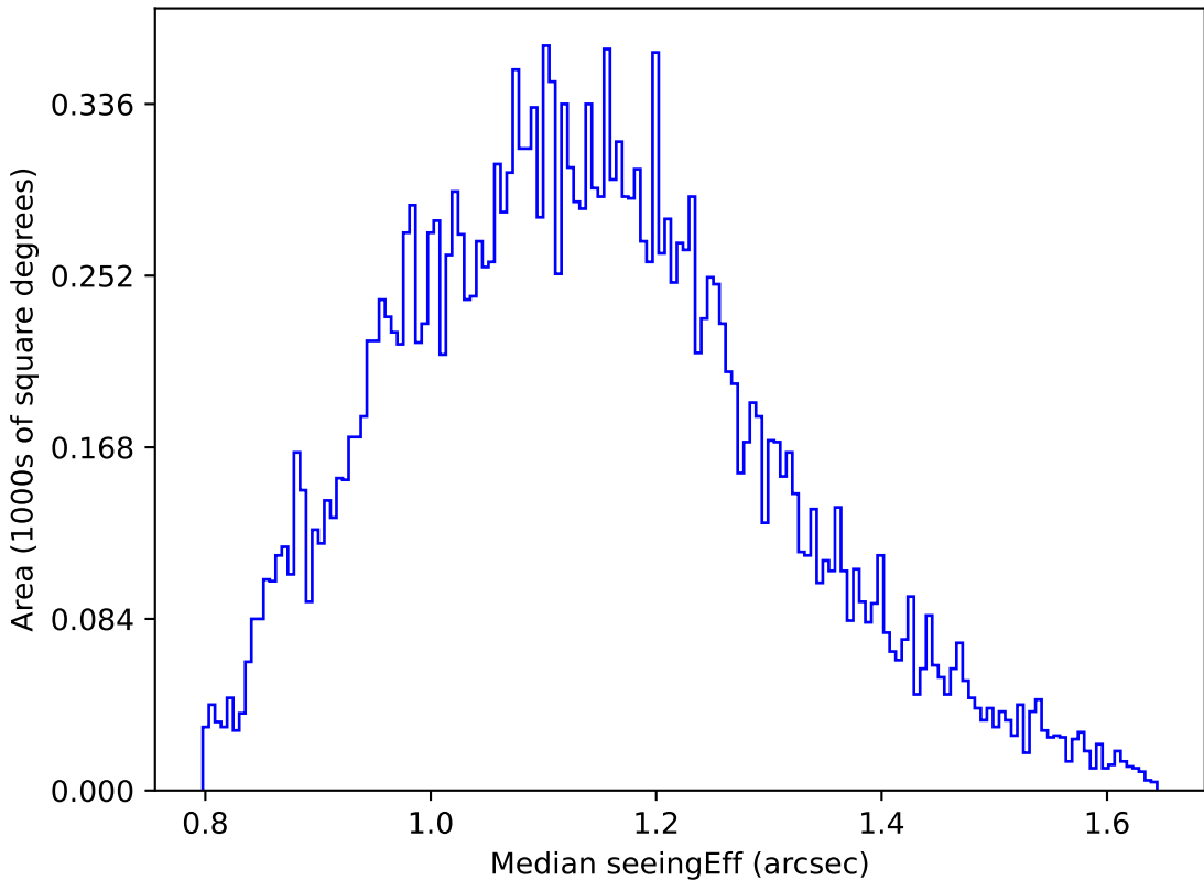
early_u_fpextra2.0_v3.4_10yrs Yr 1 u band: Median seeingEff
