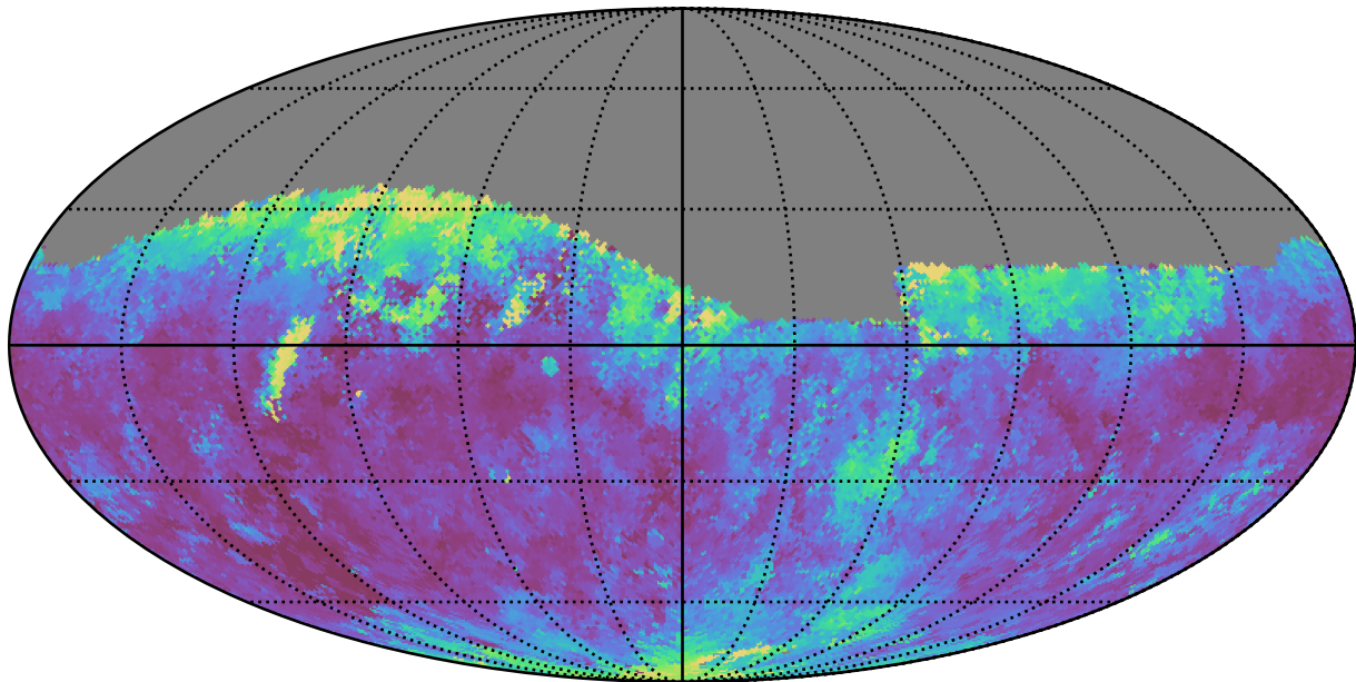
early_u_fpextra2.0_v3.4_10yrs Yr 1 r band: Median seeingEff
