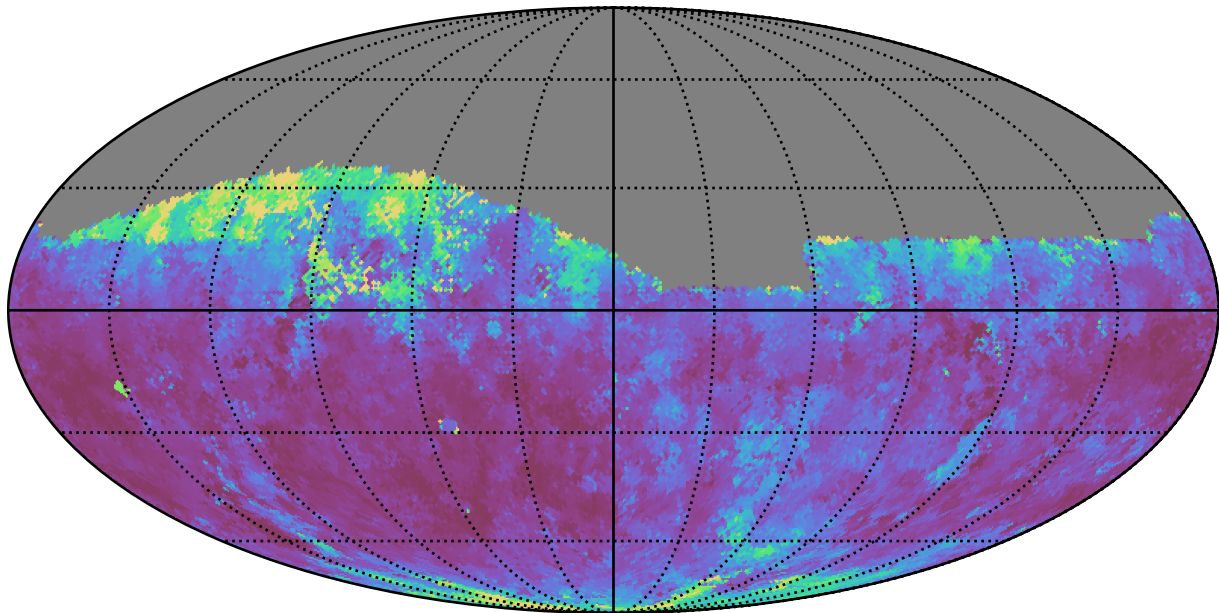
early_u_fpextra2.0_v3.4_10yrs Yr 1 i band: Median seeingEff
