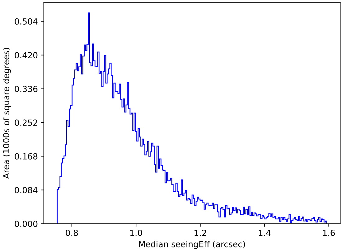
early_u_fpextra2.0_v3.4_10yrs Yr 1 i band: Median seeingEff
