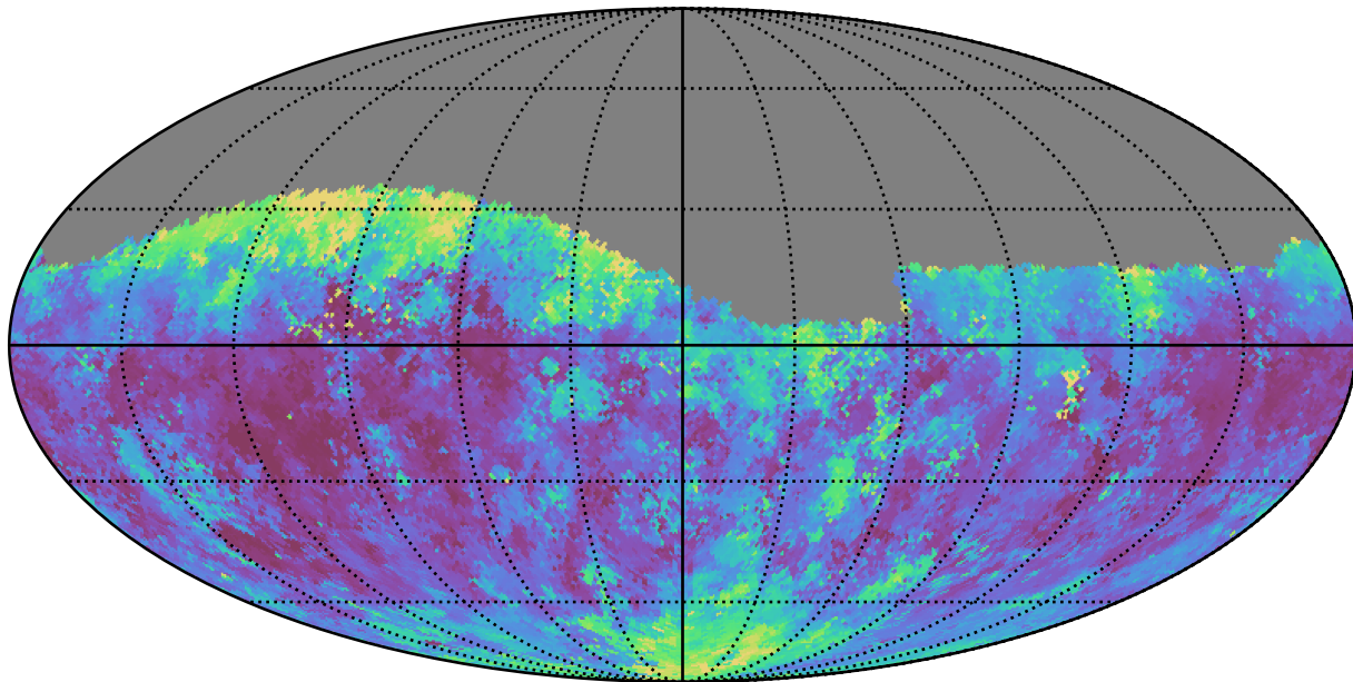
early_u_fpextra2.0_v3.4_10yrs Yr 1 g band: Median seeingEff
