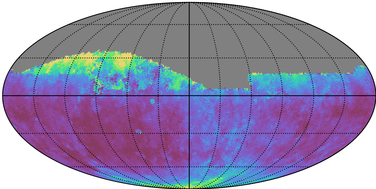
early_u_fpextra2.0_v3.4_10yrs Yr 1 all bands: Median seeingEff
