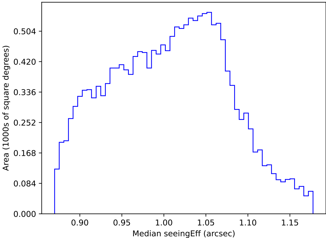
early_u_fpextra2.0_v3.4_10yrs WFD z band: Median seeingEff
