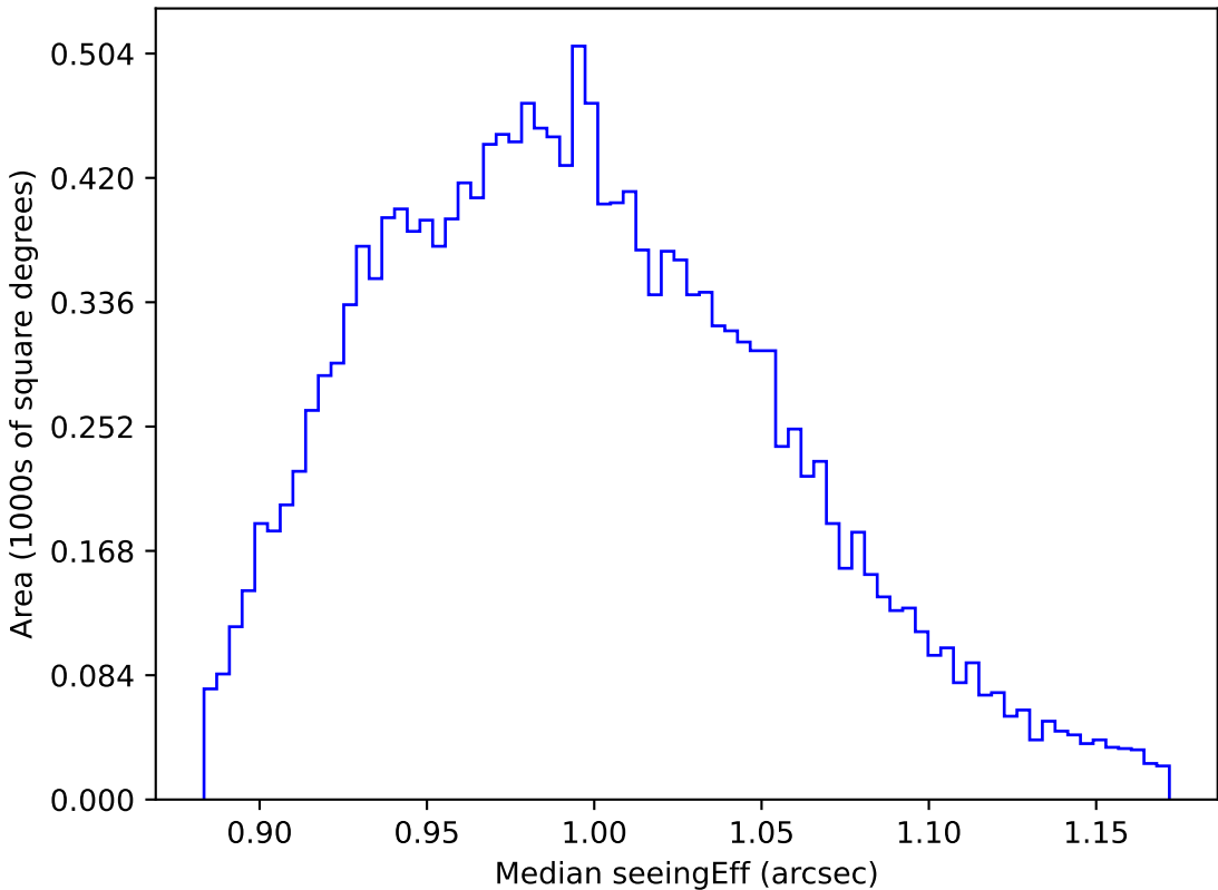
early_u_fpextra2.0_v3.4_10yrs WFD y band: Median seeingEff
