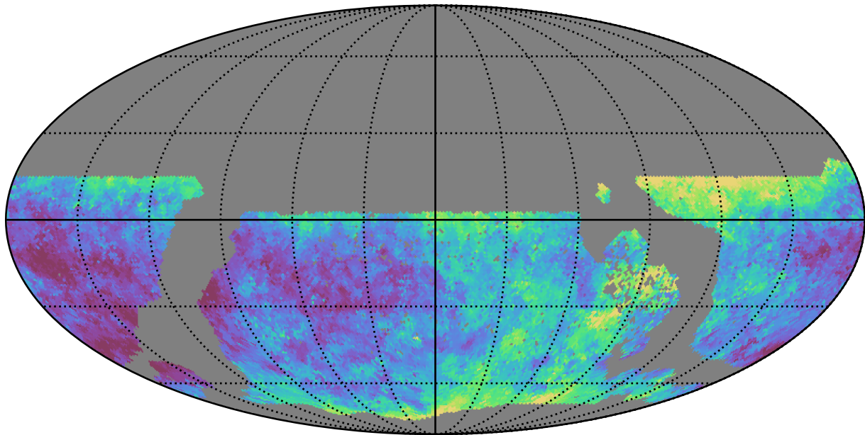
early_u_fpextra2.0_v3.4_10yrs WFD u band: Median seeingEff
