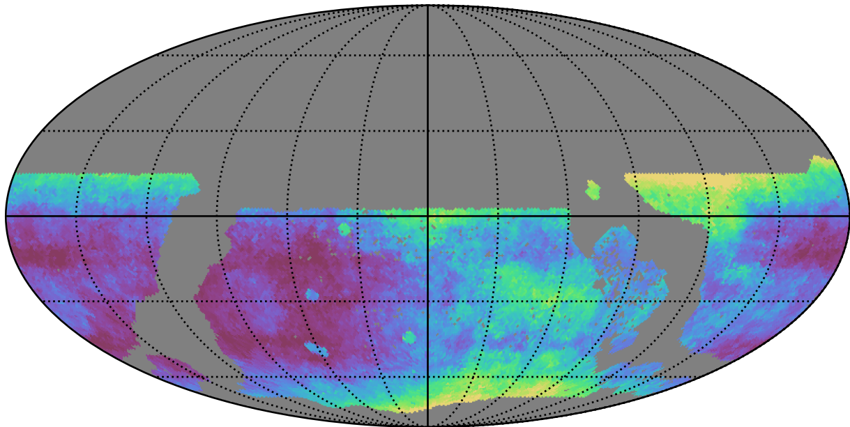
early_u_fpextra2.0_v3.4_10yrs WFD r band: Median seeingEff
