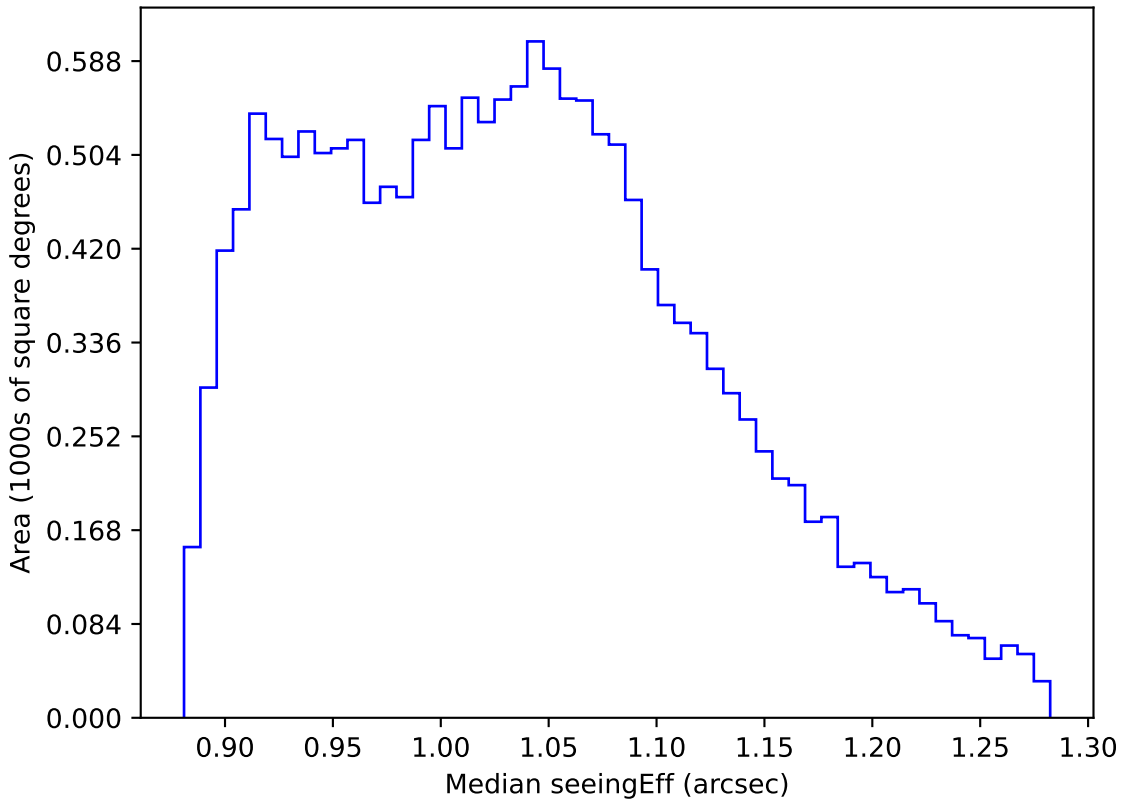
early_u_fpextra2.0_v3.4_10yrs WFD r band: Median seeingEff
