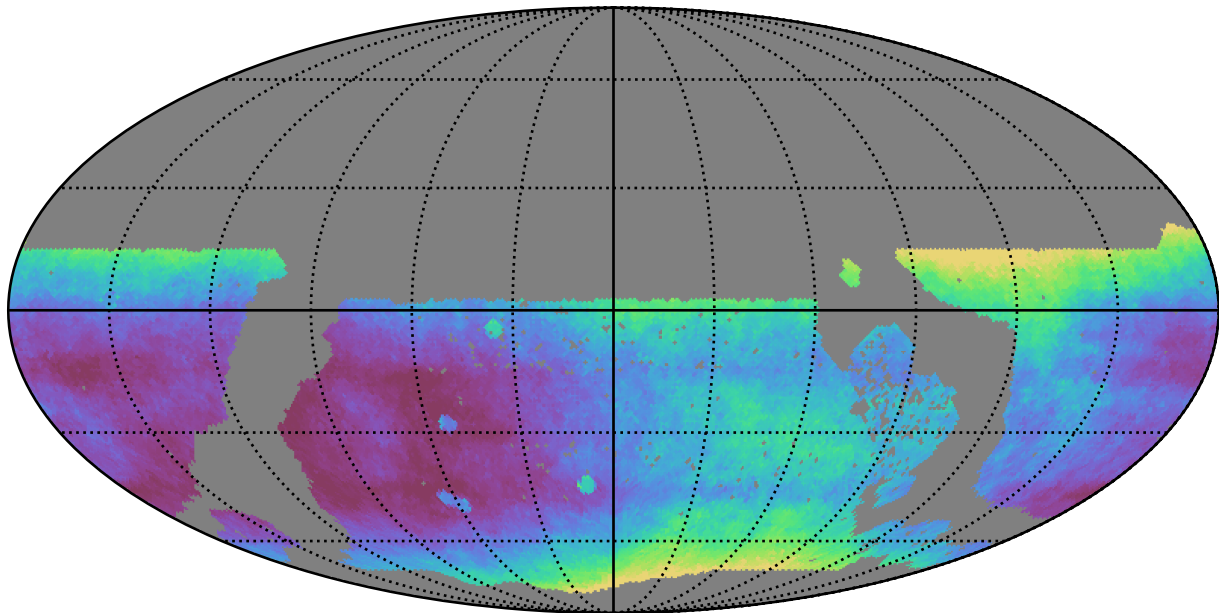
early_u_fpextra2.0_v3.4_10yrs WFD all bands: Median seeingEff
