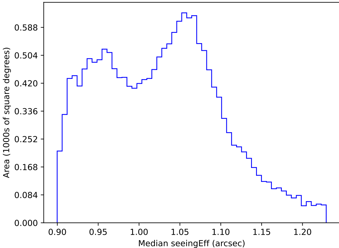
early_u_fpextra2.0_v3.4_10yrs WFD all bands: Median seeingEff
