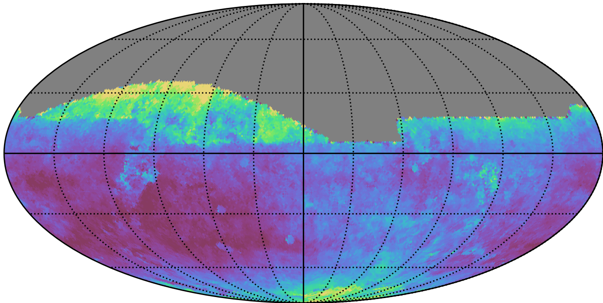
early_u_fpextra2.0_v3.4_10yrs All sky z band: Median seeingEff
