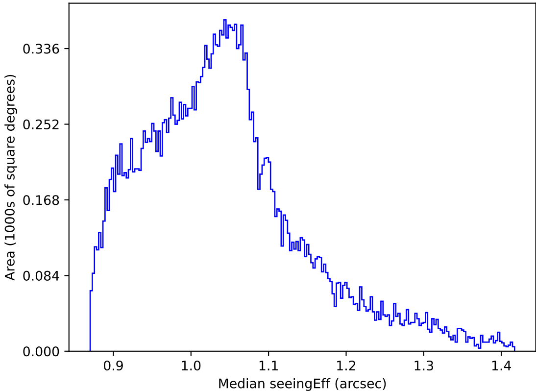
early_u_fpextra2.0_v3.4_10yrs All sky z band: Median seeingEff
