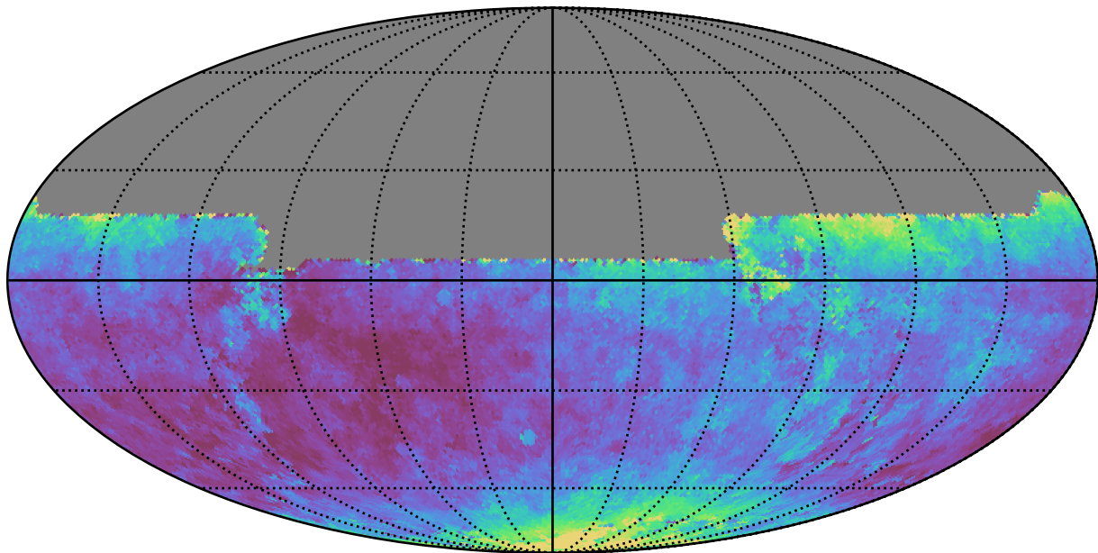
early_u_fpextra2.0_v3.4_10yrs All sky y band: Median seeingEff
