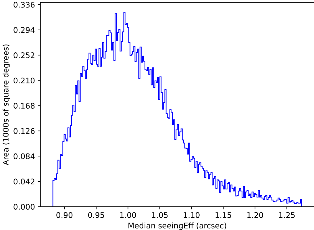
early_u_fpextra2.0_v3.4_10yrs All sky y band: Median seeingEff
