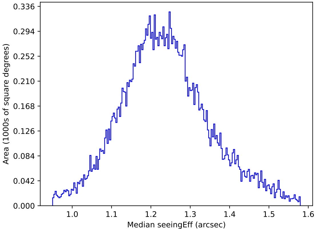
early_u_fpextra2.0_v3.4_10yrs All sky u band: Median seeingEff
