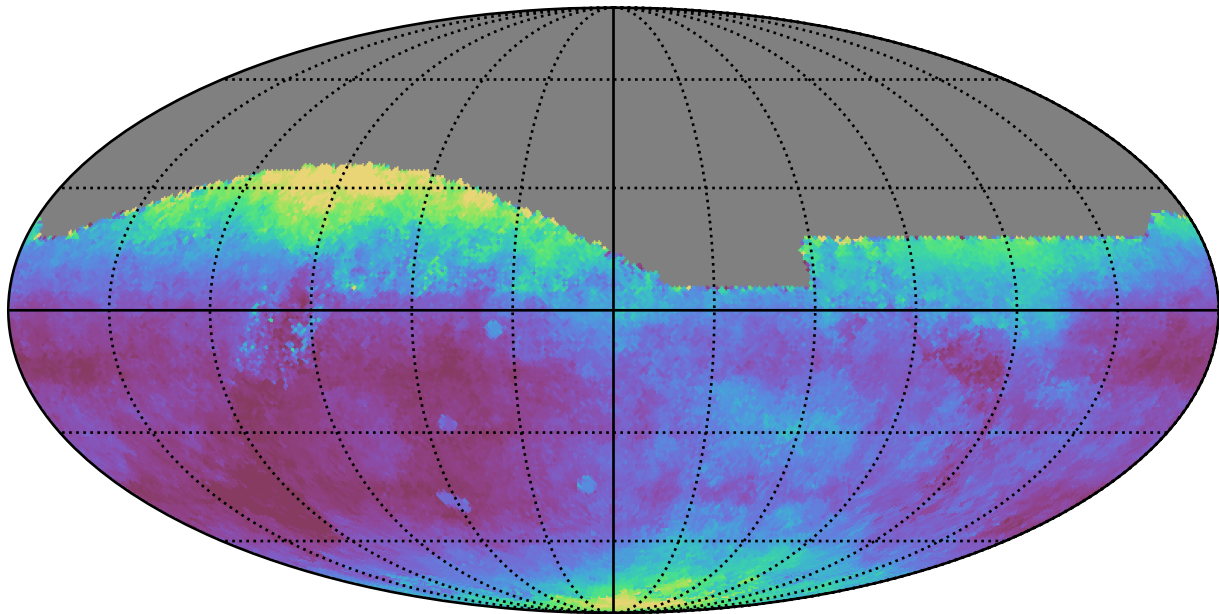
early_u_fpextra2.0_v3.4_10yrs All sky r band: Median seeingEff
