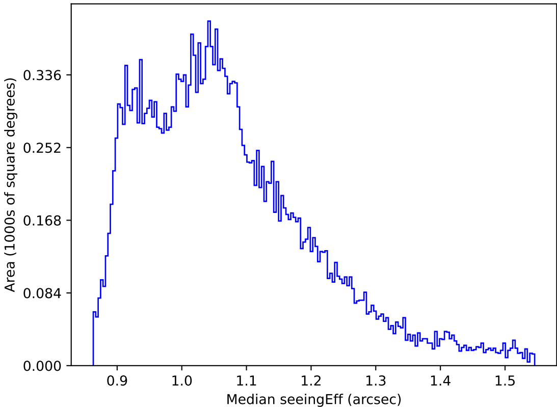
early_u_fpextra2.0_v3.4_10yrs All sky r band: Median seeingEff
