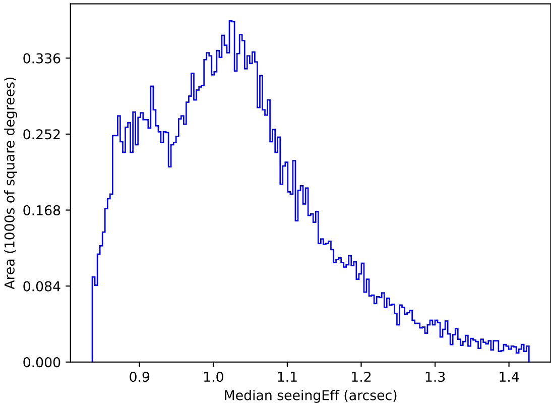
early_u_fpxextra2.0_v3.4_10yrs All sky i band: Median seeingEff
