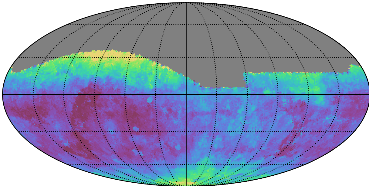
early_u_fpextra2.0_v3.4_10yrs All sky g band: Median seeingEff
