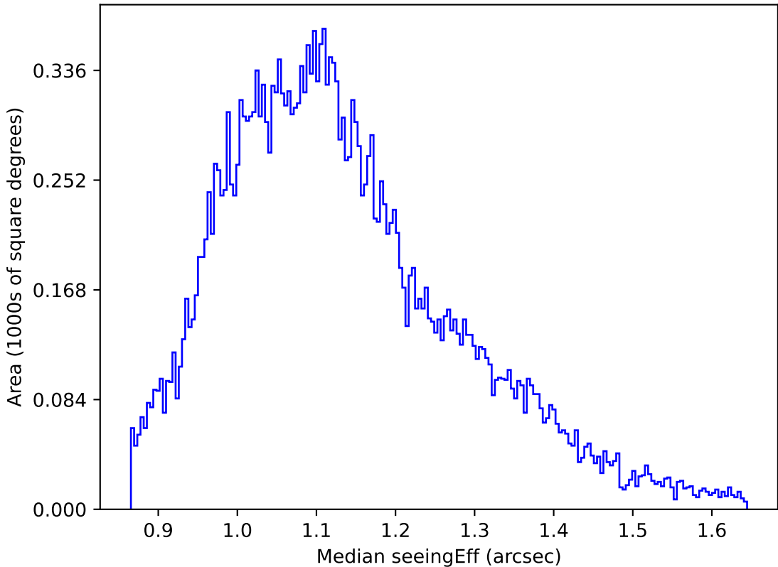
early_u_fpextra2.0_v3.4_10yrs All sky g band: Median seeingEff
