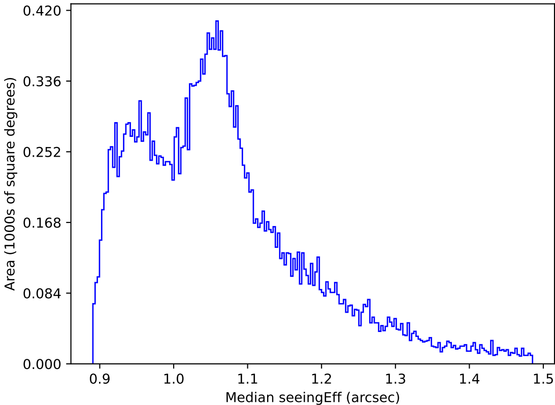
early_u_fpextra2.0_v3.4_10yrs All sky all bands: Median seeingEff
