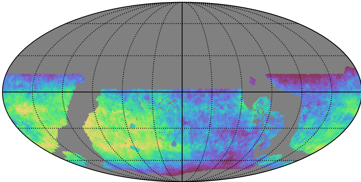
early_u_fpextra2.0_v3.4_10yrs WFD z band: Median saturation_mag
