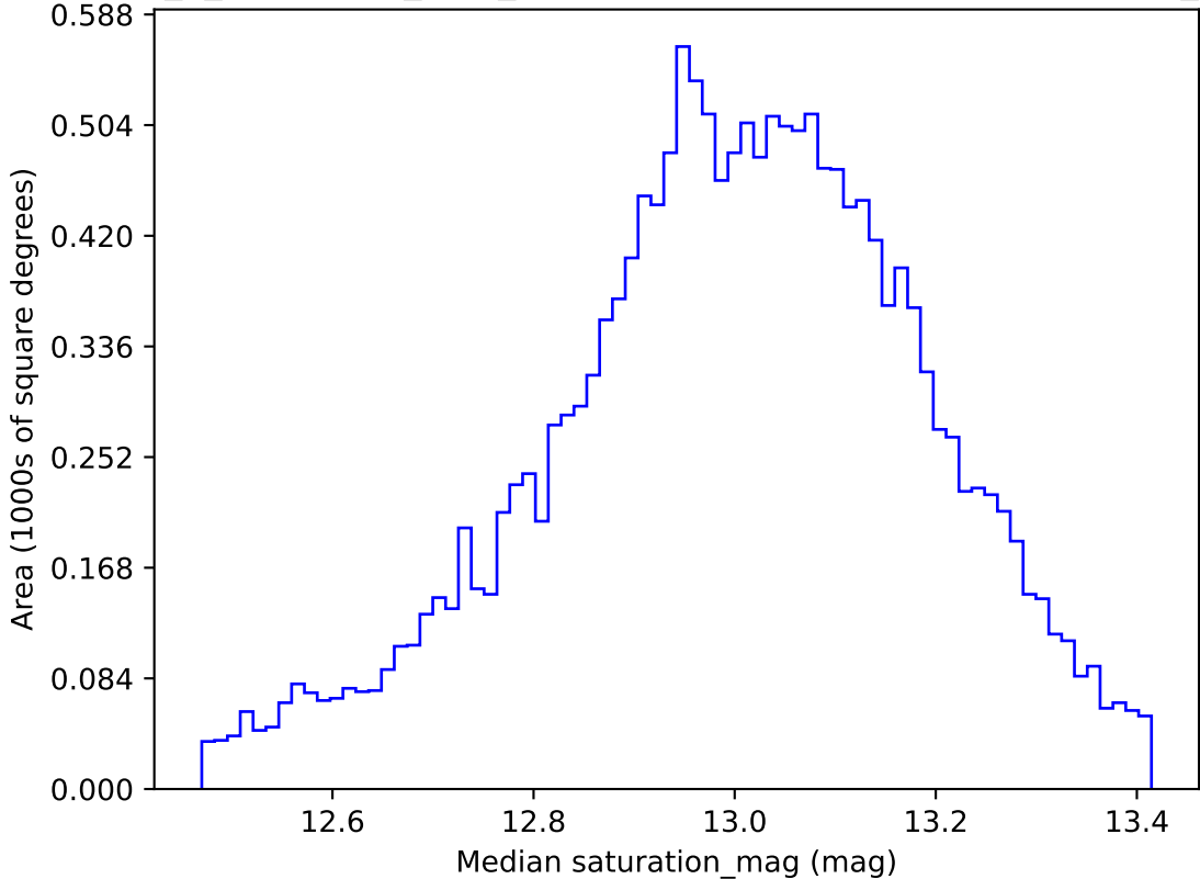
early_u_fpextra2.0_v3.4_10yrs WFD u band: Median saturation_mag
