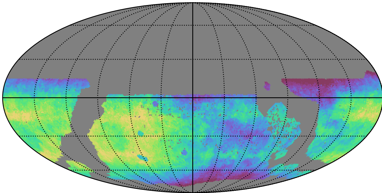
early_u_fpextra2.0_v3.4_10yrs WFD r band: Median saturation_mag
