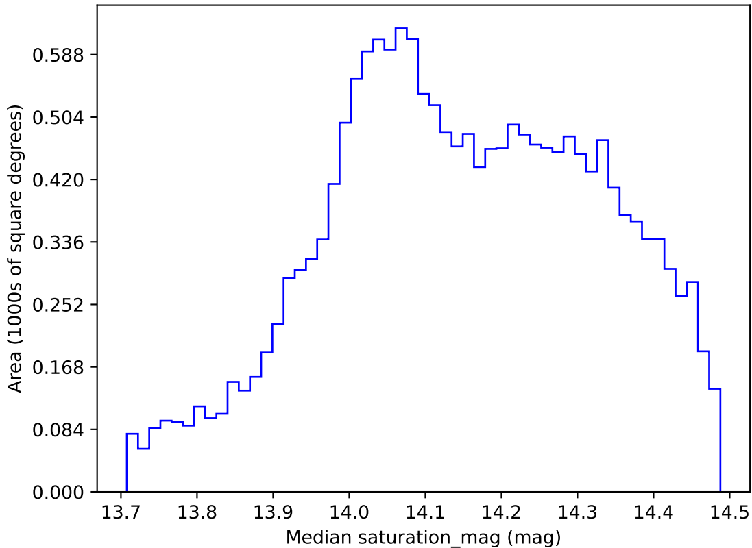
early_u_fpextra2.0_v3.4_10yrs WFD all bands: Median saturation_mag
