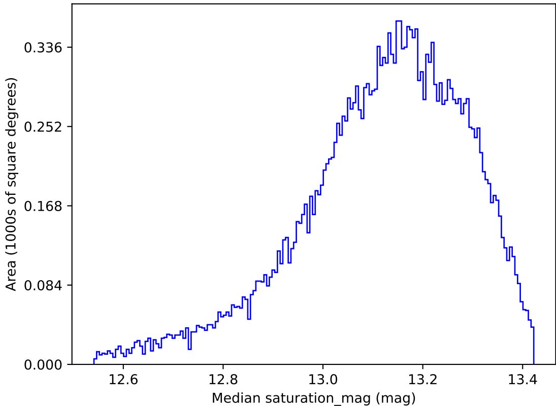
early_u_fpextra2.0_v3.4_10yrs All sky y band: Median saturation_mag
