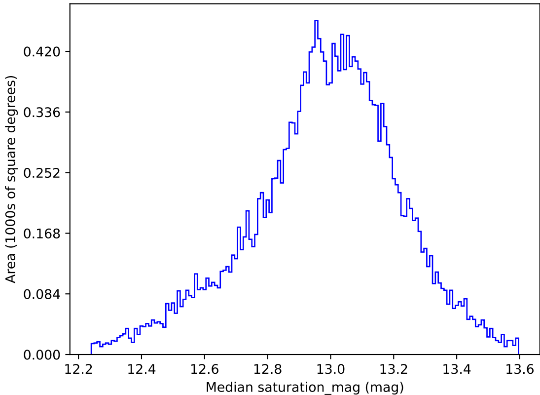
early_u_fpextra2.0_v3.4_10yrs All sky u band: Median saturation_mag
