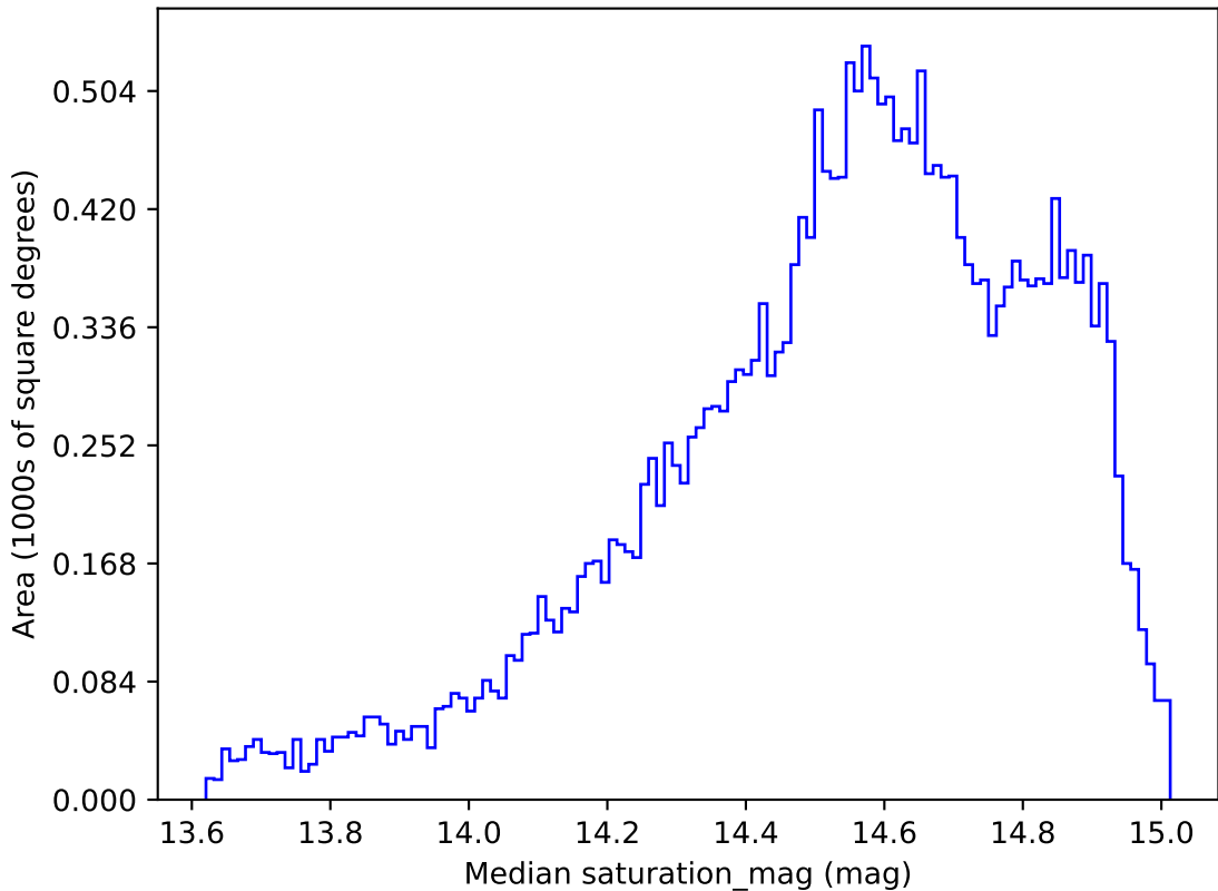
early_u_fpextra2.0_v3.4_10yrs All sky r band: Median saturation_mag
