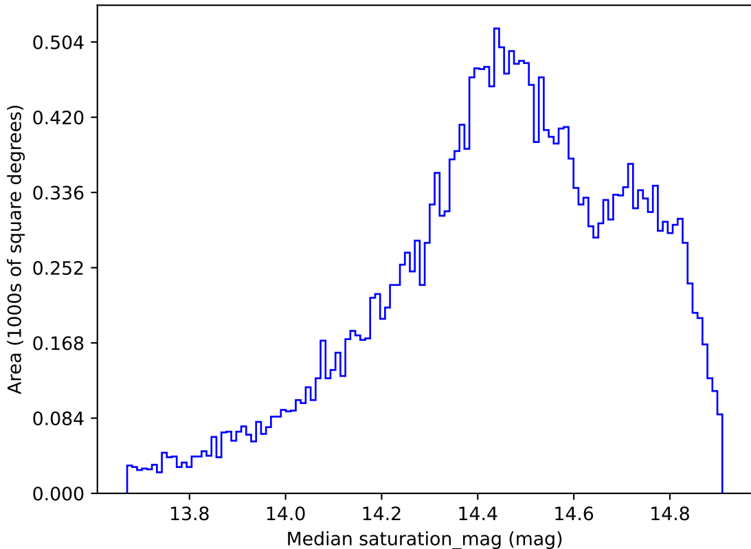
early_u_fpextra2.0_v3.4_10yrs All sky i band: Median saturation_mag
