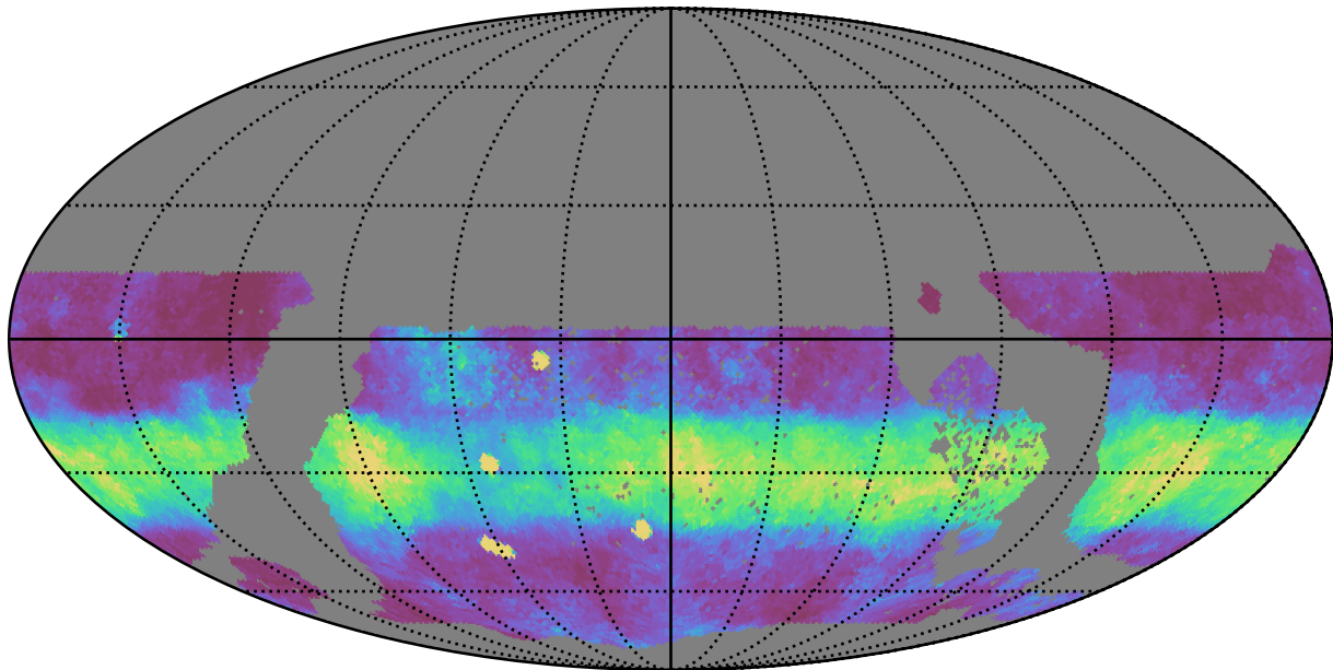
early_u_fpextra2.0_v3.4_10yrs WFD z band: Median normairmass
