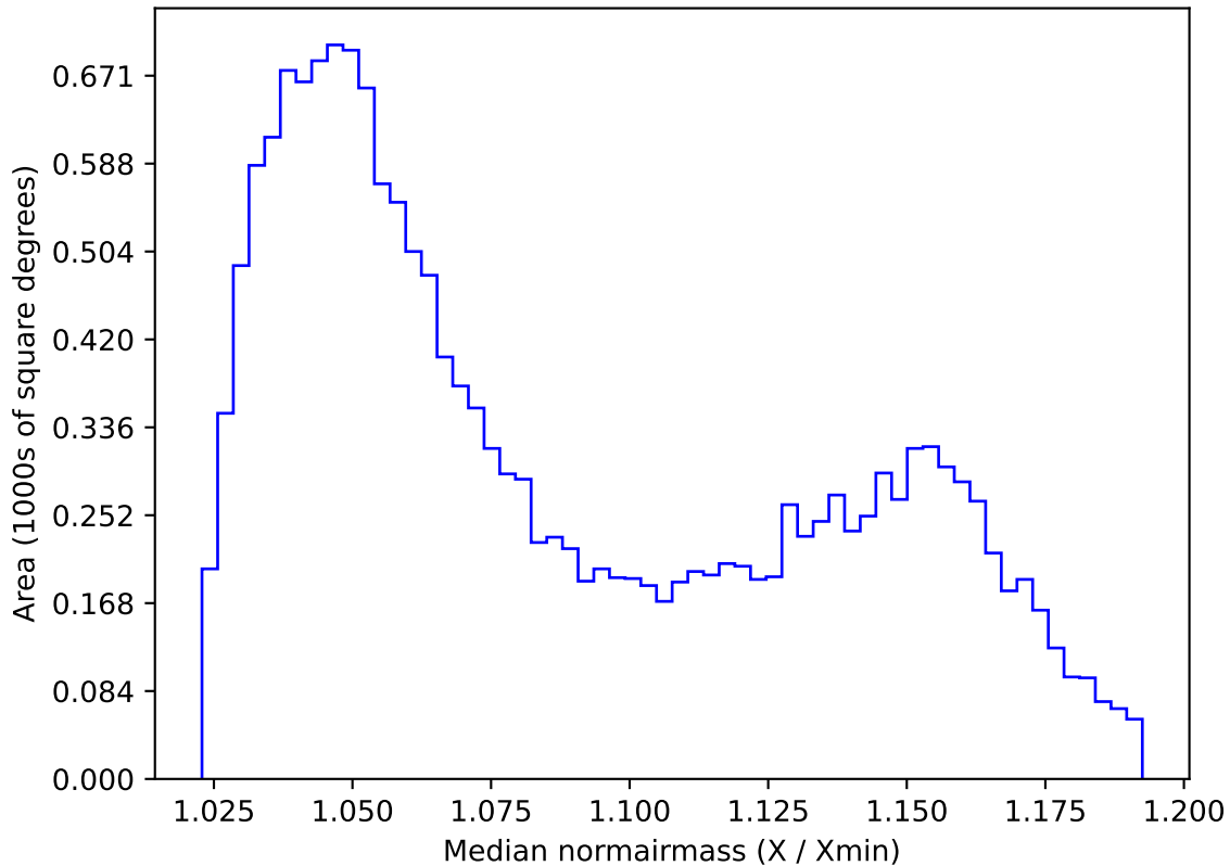
early_u_fpextra2.0_v3.4_10yrs WFD z band: Median normairmass
