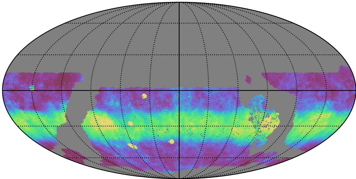
early_u_fpextra2.0_v3.4_10yrs WFD y band: Median normairmass
