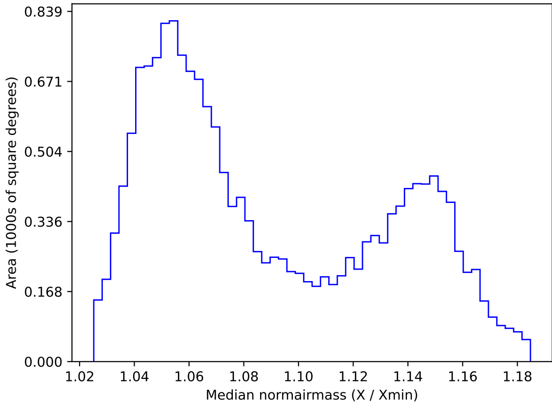
early_u_fpextra2.0_v3.4_10yrs WFD y band: Median normairmass
