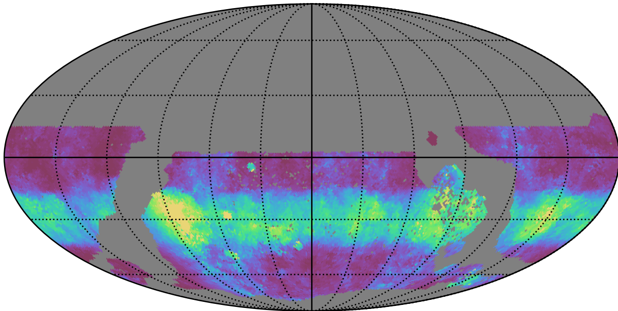
early_u_fpextra2.0_v3.4_10yrs WFD u band: Median normairmass
