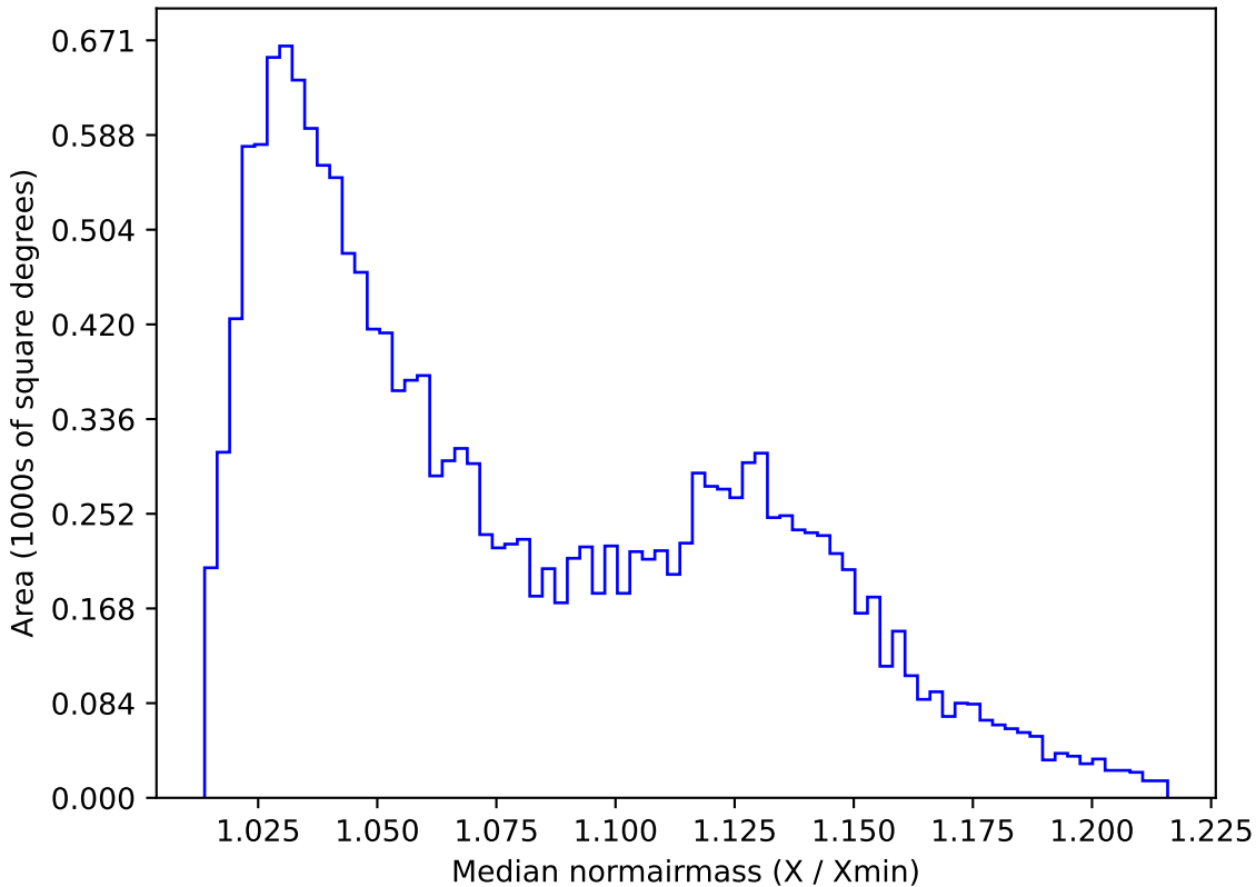
early_u_fpextra2.0_v3.4_10yrs WFD u band: Median normairmass
