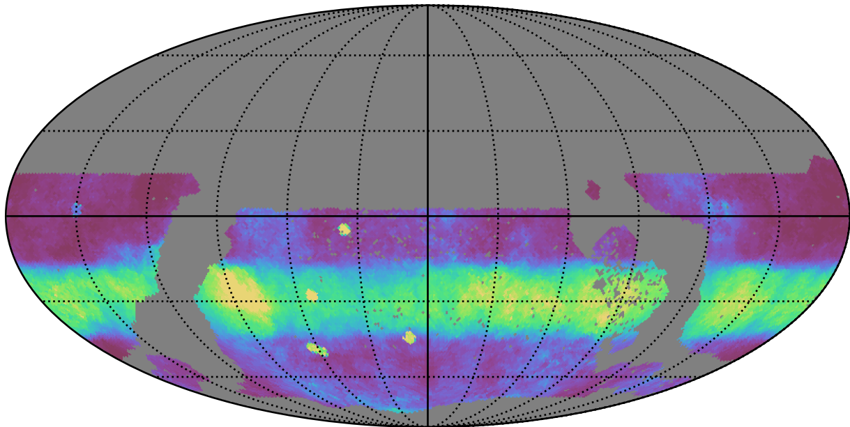
early_u_fpextra2.0_v3.4_10yrs WFD r band: Median normairmass
