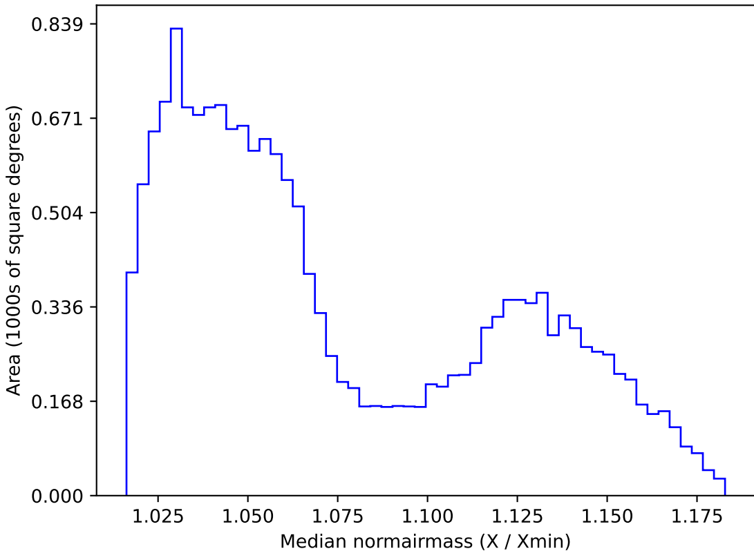
early_u_fpextra2.0_v3.4_10yrs WFD r band: Median normairmass
