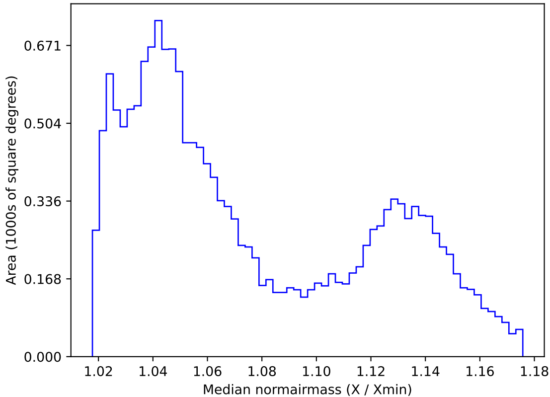
early_u_fpextra2.0_v3.4_10yrs WFD i band: Median normairmass
