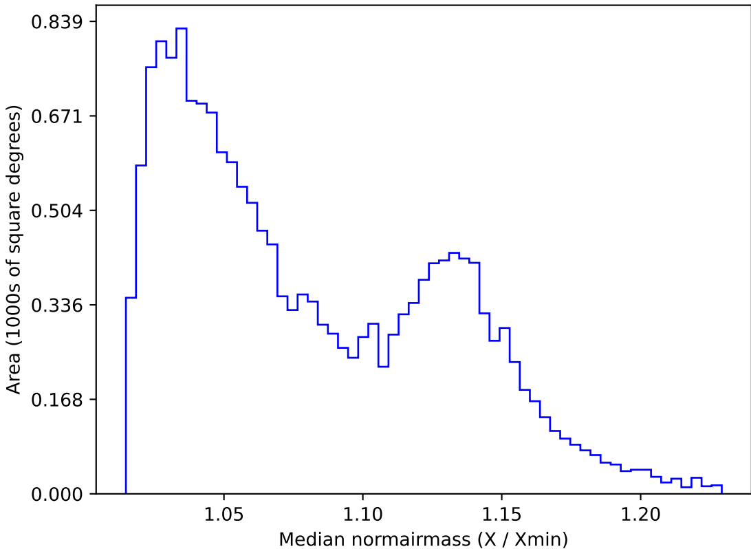
early_u_fpextra2.0_v3.4_10yrs WFD g band: Median normairmass
