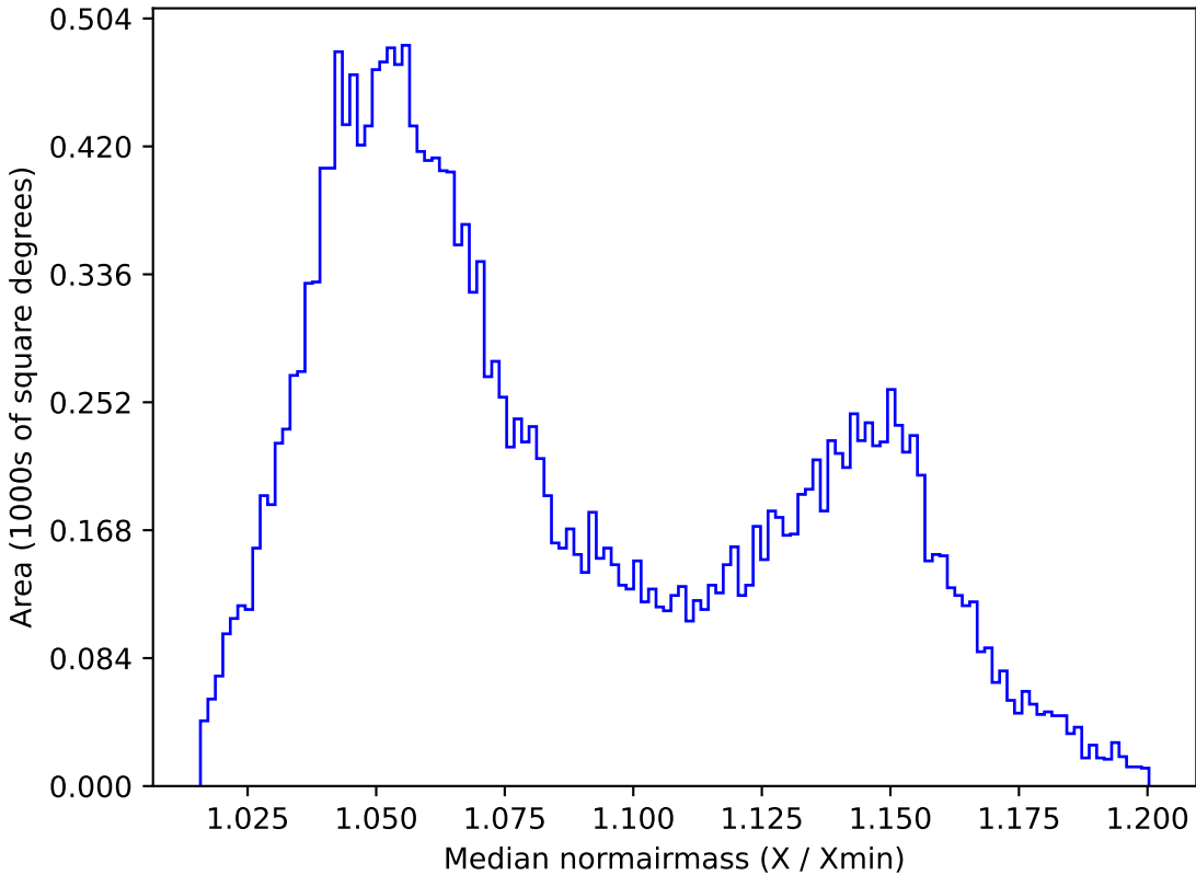
early_u_fpextra2.0_v3.4_10yrs All sky y band: Median normairmass
