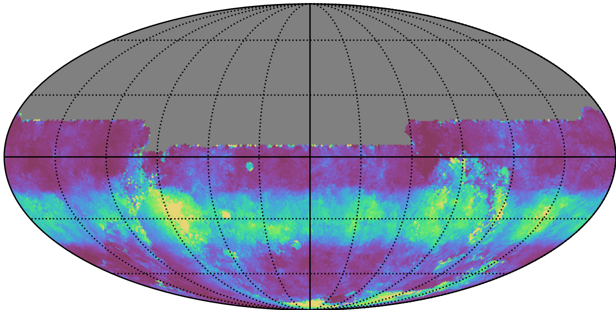
early_u_fpextra2.0_v3.4_10yrs All sky u band: Median normairmass
