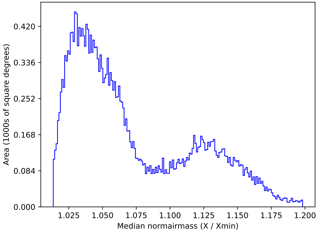
early_u_fpextra2.0_v3.4_10yrs All sky r band: Median normairmass
