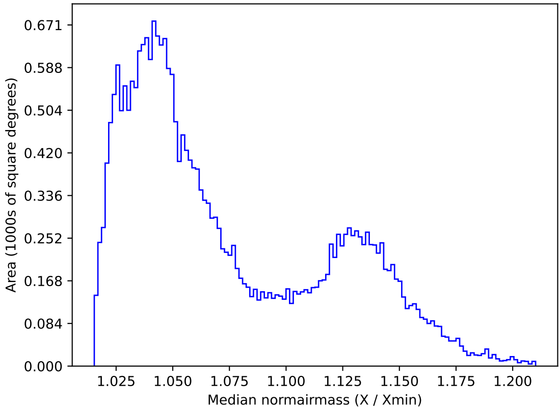
early_u_fpextra2.0_v3.4_10yrs All sky i band: Median normairmass
