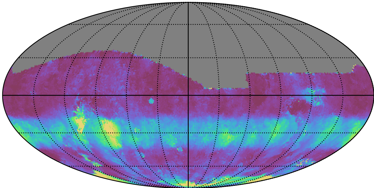
early_u_fpextra2.0_v3.4_10yrs All sky g band: Median normairmass
